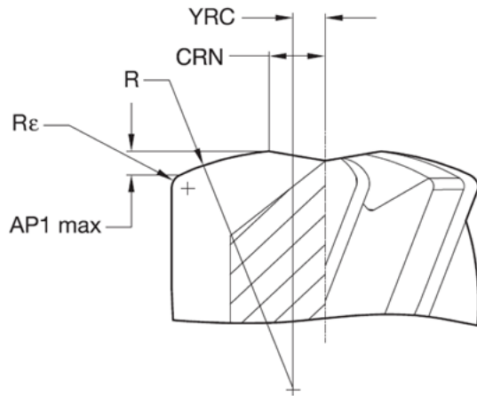
FH200-H Schematic Diagram of the End Edge of 6 Flute Corner Radius Endmill
