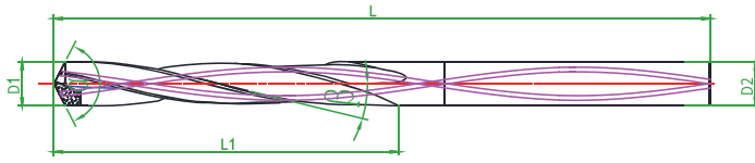
PCD twist drill-- Metric(with internal coolant)
