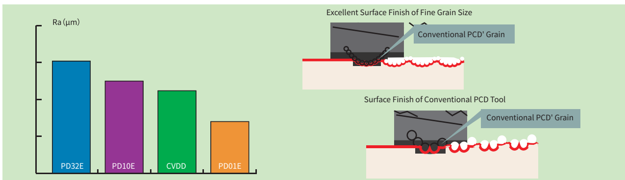
(Effect of grain size on finish machining surface)
